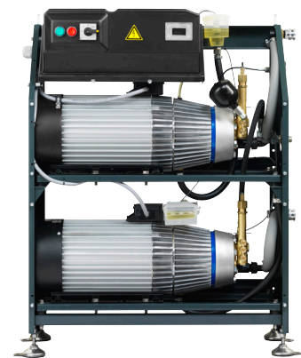
Cabinet can be removed quickly for direct access to the motor pump
