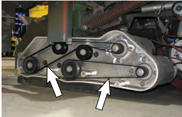
Dual Force Sweeping Drive Belts
